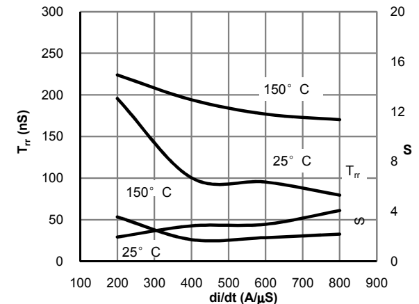
Fig 25: Diode Reverse Recovery Time and Softness Factor vs. di/dt ( V_{GE}=15V, V_{CE}=400V, I_F=15A )
