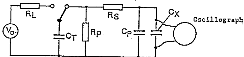
Impulse Voltage Test Circuit
