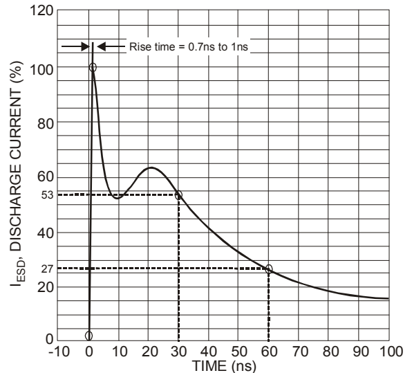
Figure 6 ESD Discharge Current Wave Form IEC 6100-4-2 (330Ω/150pF)
