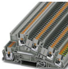
Installation ground terminal block, Push-in connection, cross section: 0.14 mm 2 - 4 mm 2 , AWG: 26 - 12, width: 5.2 mm, color: gray, mounting type: NS 35/7,5, NS 35/15
