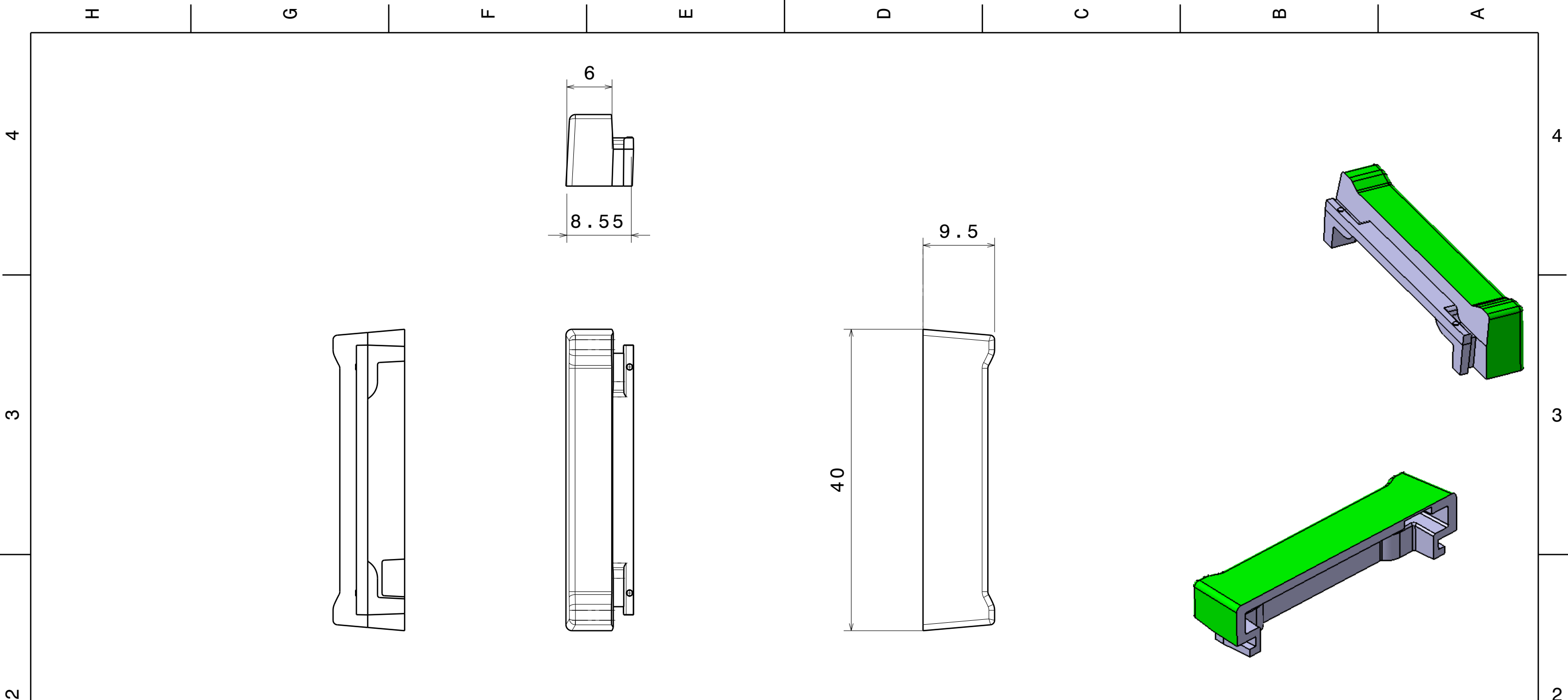
Section B-B (2:1)
