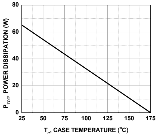
Figure 4. Power Derating
