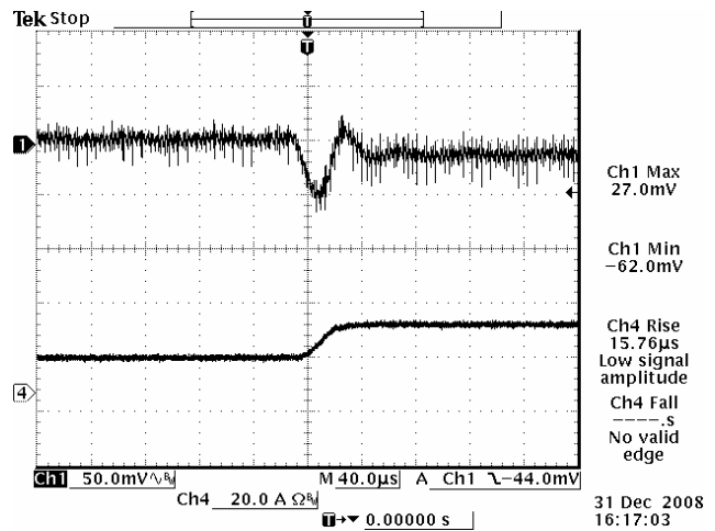
50% to 75% Load Transients
