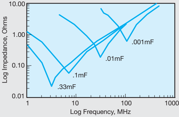
Impedance vs. Frequency Effect of Capacitance – AVX SpinGuards
