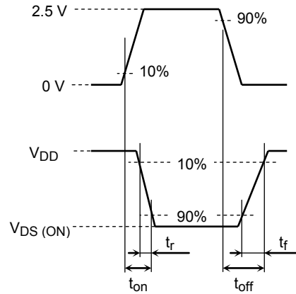
(c) V_{OUT}
