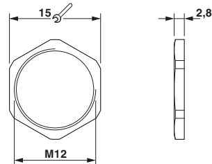
Dimensional drawing
