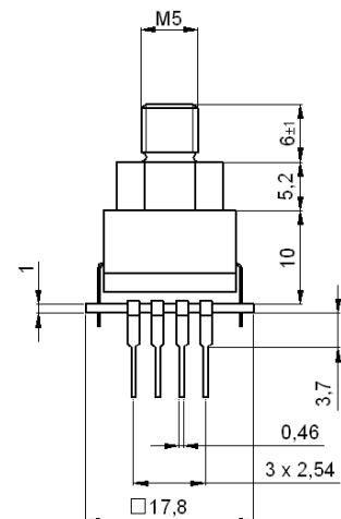
Type KC for gauge pressure (M5 thread connection)
