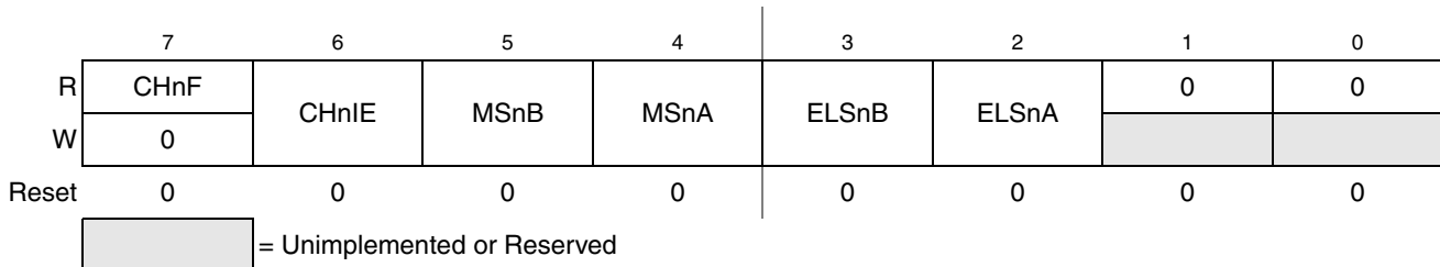
Figure 13-12. TPM Channel n Status and Control Register (TPMxCnSC)
