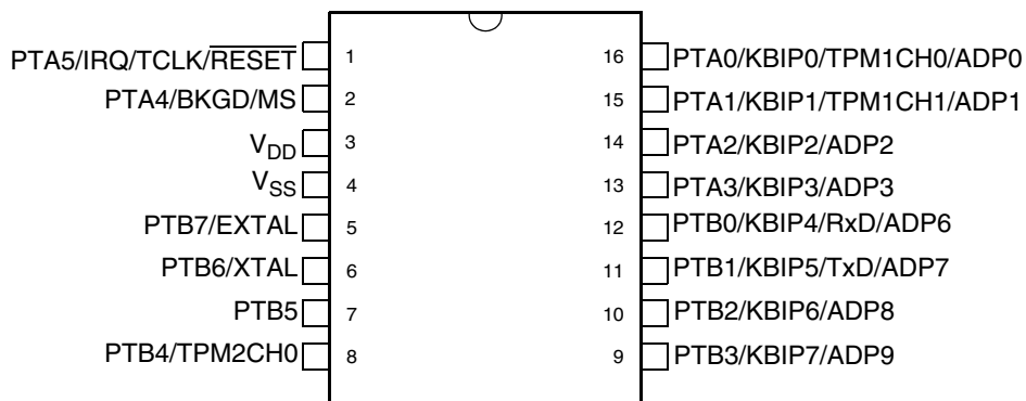
Figure 2-2. MC9S08SE8 in 16-Pin TSSOP Package
