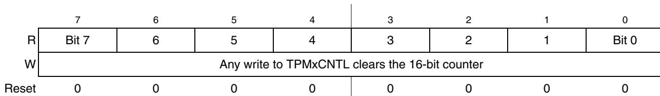
Figure 13-9. TPM Counter Register Low (TPMxCNTL)
