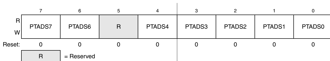
Figure 6-6. Drive Strength Selection for Port A Register (PTADS)
