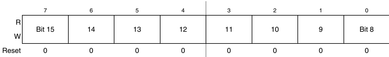
Figure 13-10. TPM Counter Modulo Register High (TPMxMODH)
