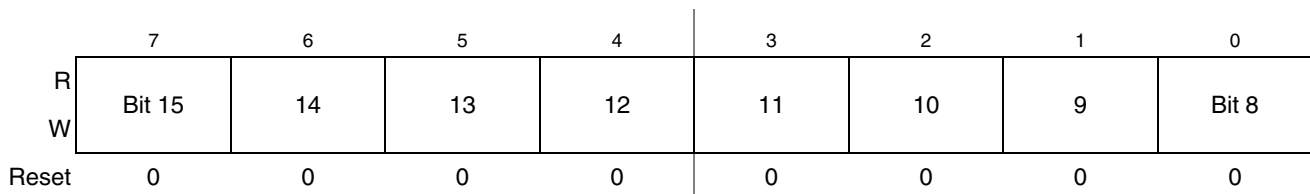
Figure 13-13. TPM Channel Value Register High (TPMxCnVH)
