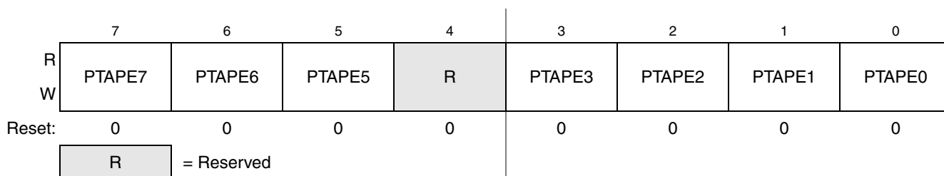
Figure 6-4. Internal Pull Enable for Port A Register (PTAPE)
