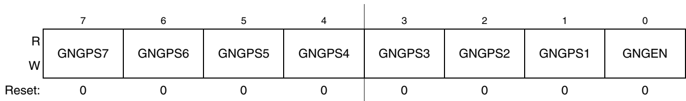
Figure 6-17. Ganged Output Drive Control Register (GNGC)
