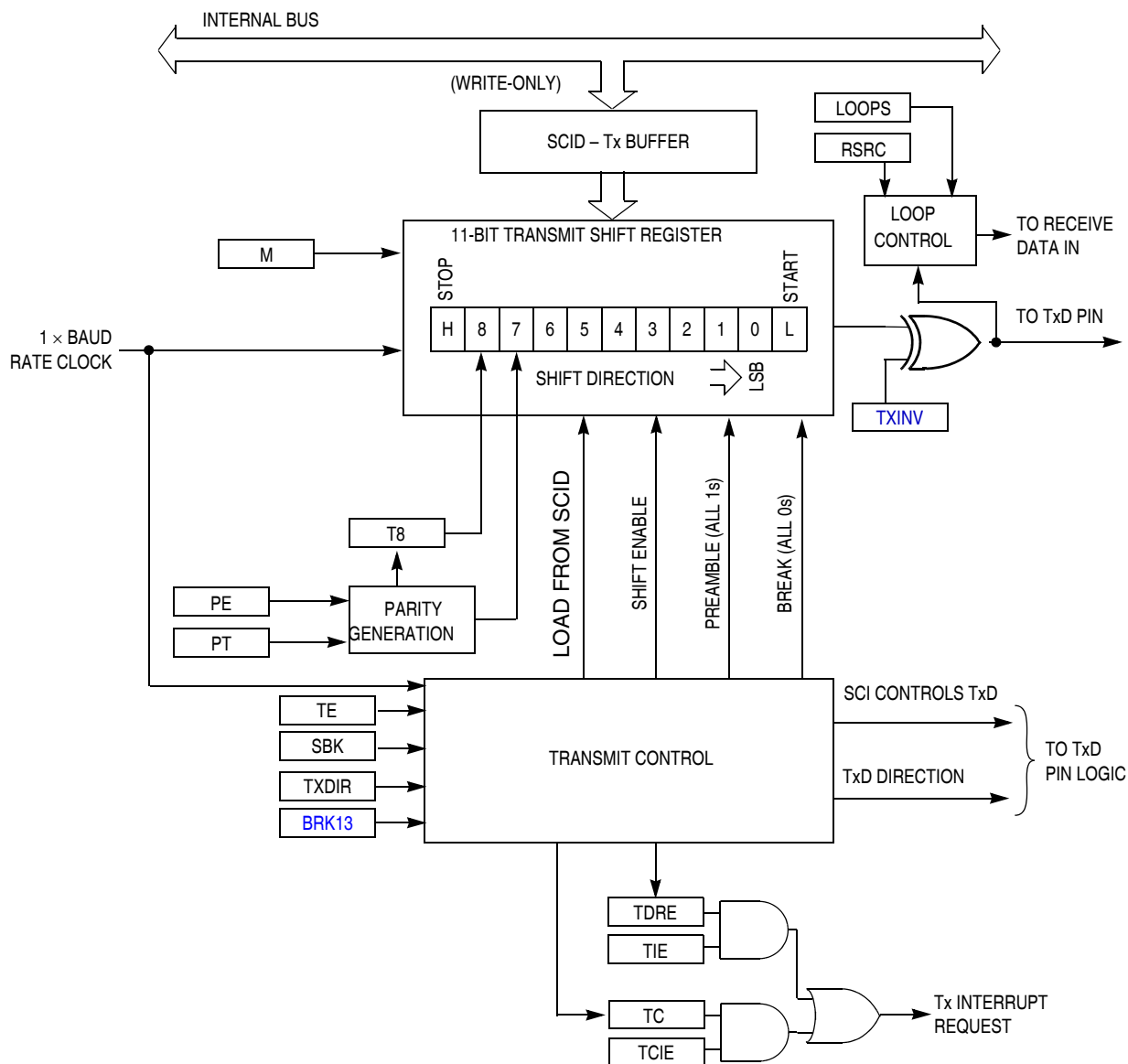
Figure 12-2. SCI Transmitter Block Diagram
