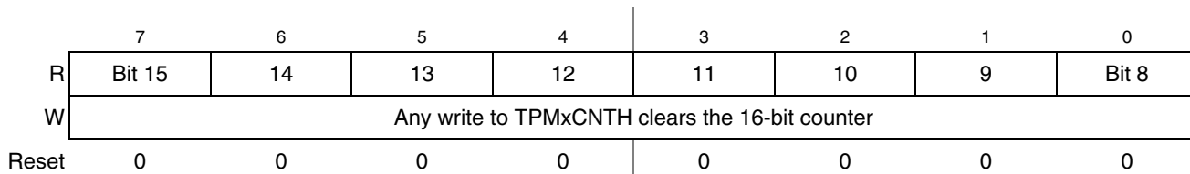
Figure 13-8. TPM Counter Register High (TPMxCNTH)
