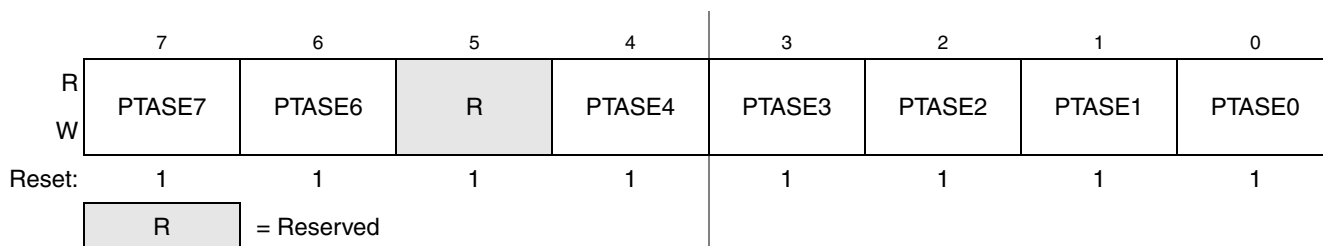
Figure 6-5. Slew Rate Enable for Port A Register (PTASE)
