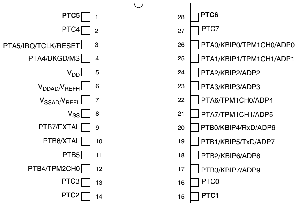
Figure 2-1. MC9S08SE8 in 28-Pin SOIC/PDIP Package
