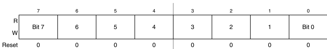
Figure 13-14. TPM Channel Value Register Low (TPMxCnVL)
