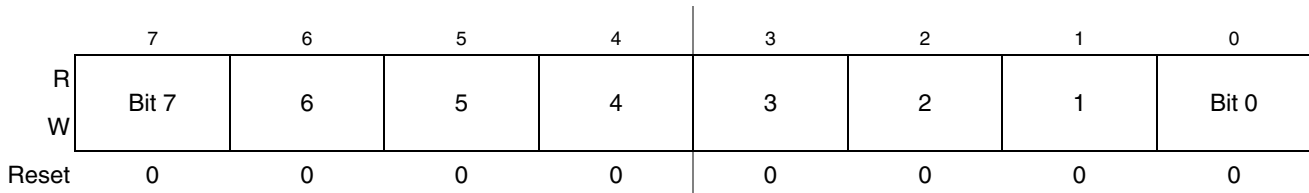
Figure 13-11. TPM Counter Modulo Register Low (TPMxMODL)
