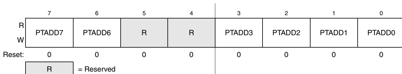
Figure 6-3. Port A Data Direction Register (PTADD)
