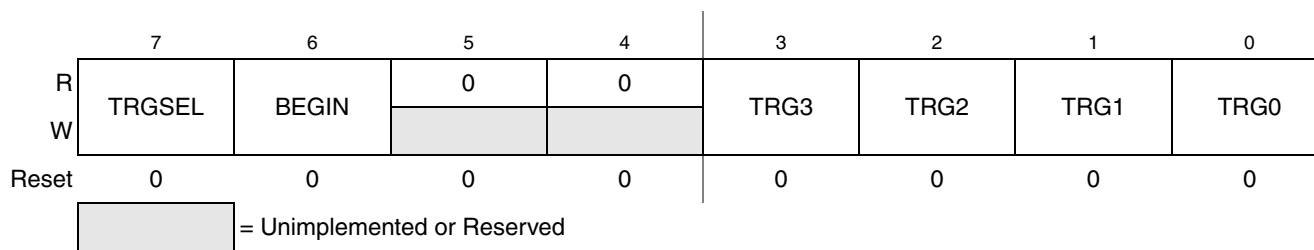
Figure 14-8. Debug Trigger Register (DBGT)
