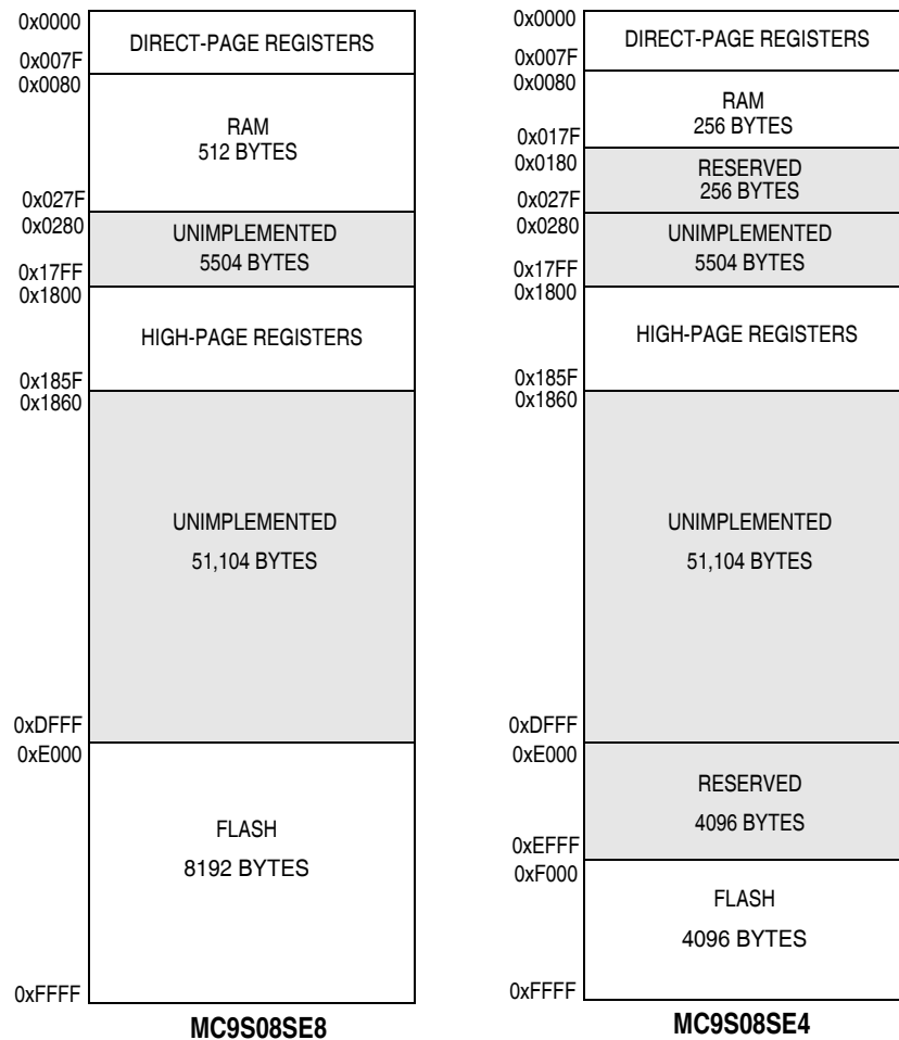
Figure 4-1. MC9S08SE8/4 Memory Map
