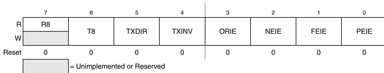
Figure 12-10. SCI Control Register 3 (SCIC3)
