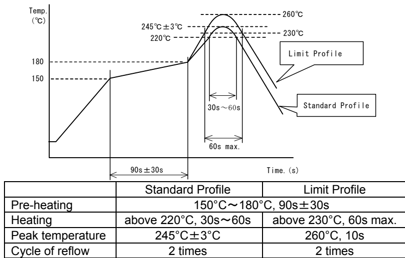
Soldering Profile for Lead Free solder
