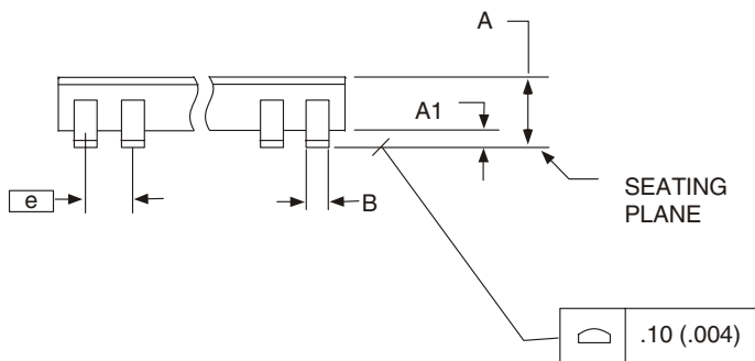
150 mil (Narrow Body) SOIC
