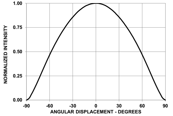
Figure 5: Radiation Pattern
