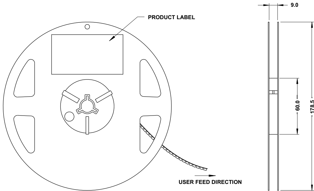
Figure 17: Reel Dimensions
