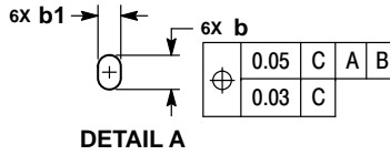
DETAIL A
