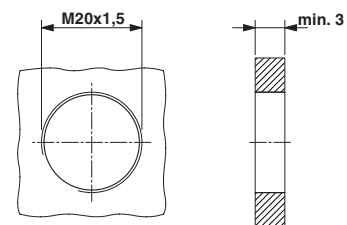
Dimensioned drawing
