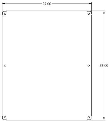
INNER PANEL
