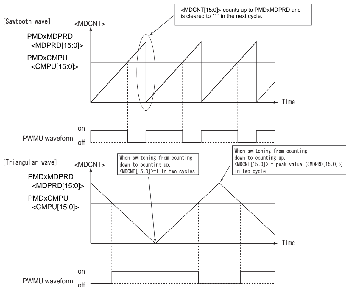
Figure 11-4 PWM Waveforms
