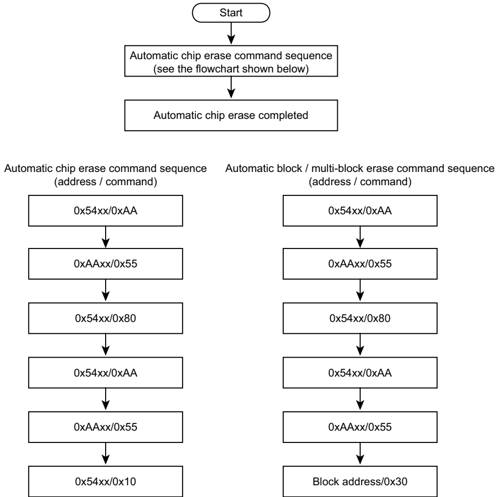
Figure 19-11 Automatic Erase
