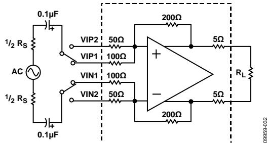
Figure 30. Basic Structure
