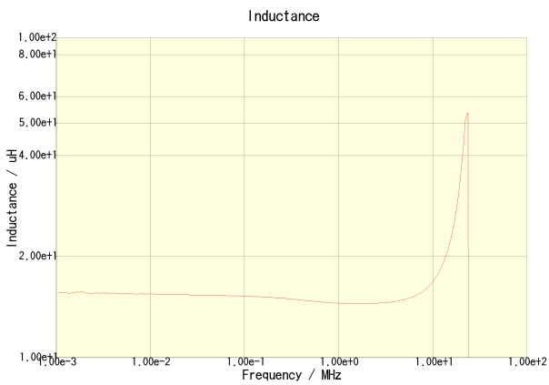
CLF6045T-150M-CA
