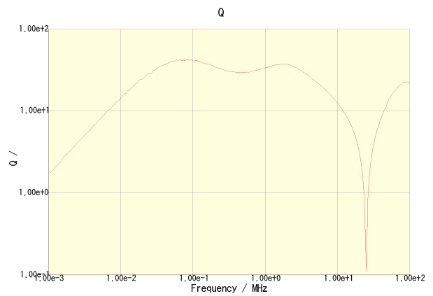
CLF6045T-150M-CA
