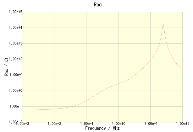
CLF6045T-150M-CA
