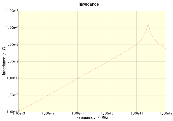
CLF6045T-150M-CA
